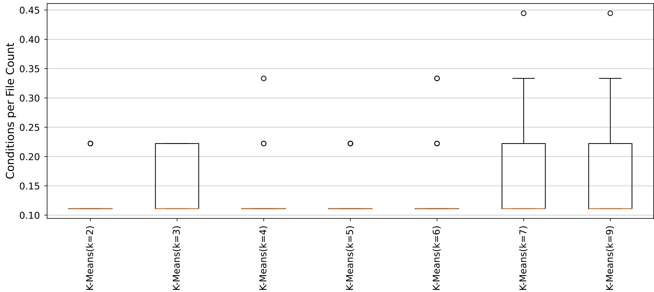
YARA Rules Conditions per File Count Distribution (Cluster14_Size9 dataset)
